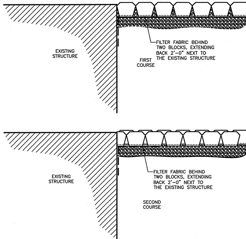
X WX ANCHOR DIAMOND® WALL ABUTTING EXISTING STRUCTURE (SCALE: 3/8" = 1'-0")
