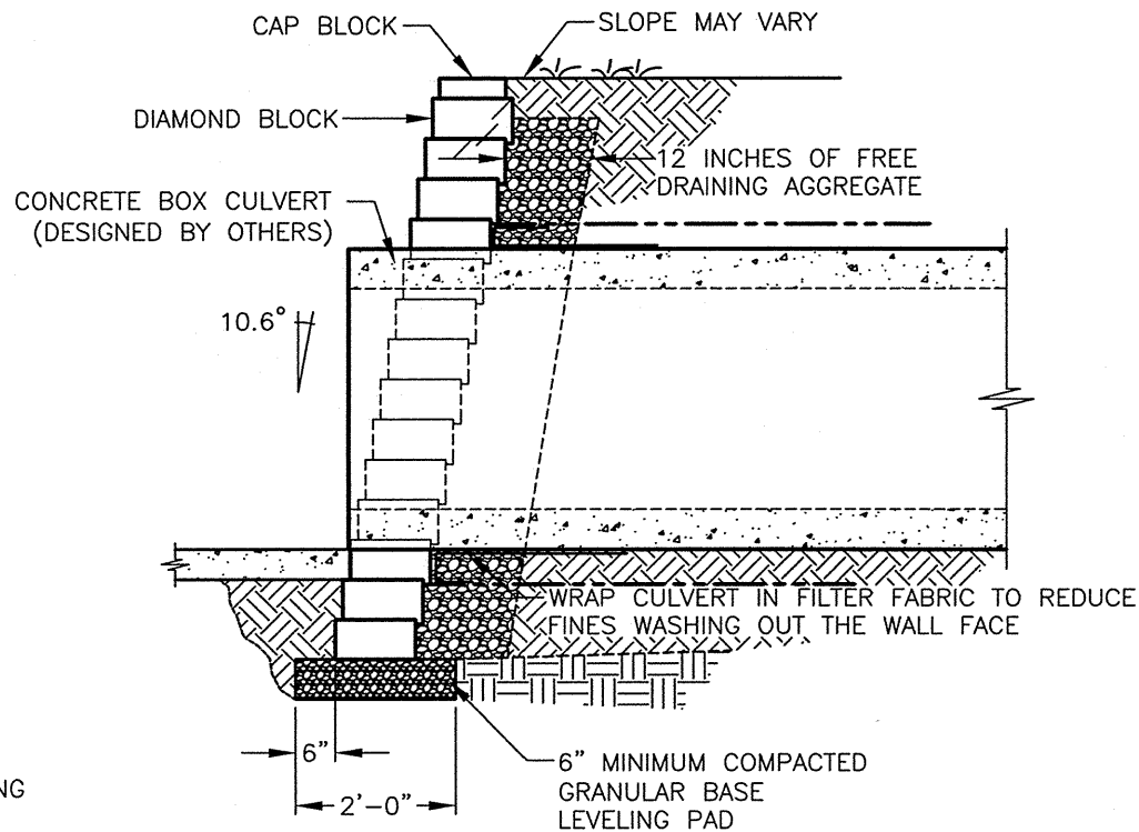
SIDE VIEW
