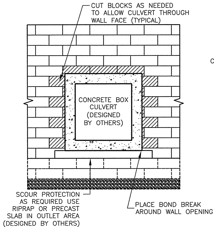
FACE VIEW
