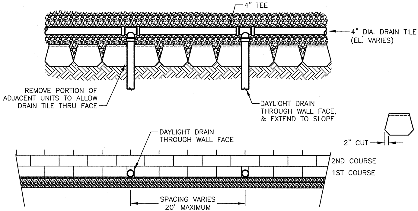
ANCHOR DIAMOND ® DAYLIGHT DRAINTILE THROUGH TOE SLOPE X WX (NOT TO SCALE)
