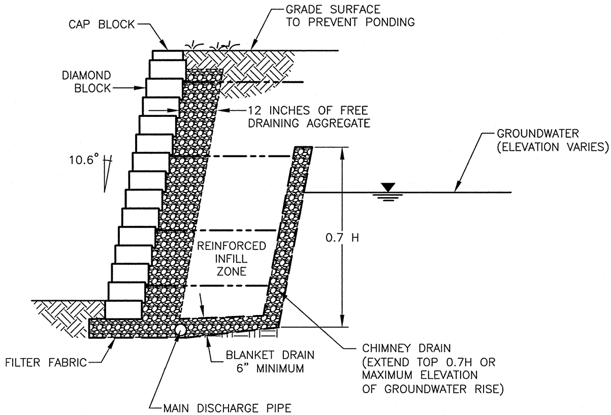
ANCHOR DIAMOND ® X POTENTIAL GROUNDWATER BEHIND WALL WX (SCALE: 3/8" = 1'-0")
