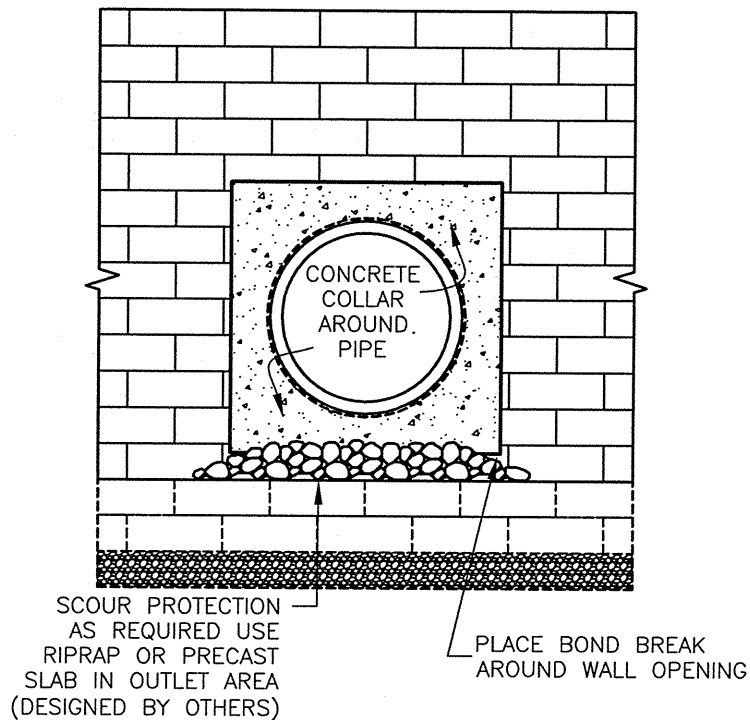
FACE VIEW
