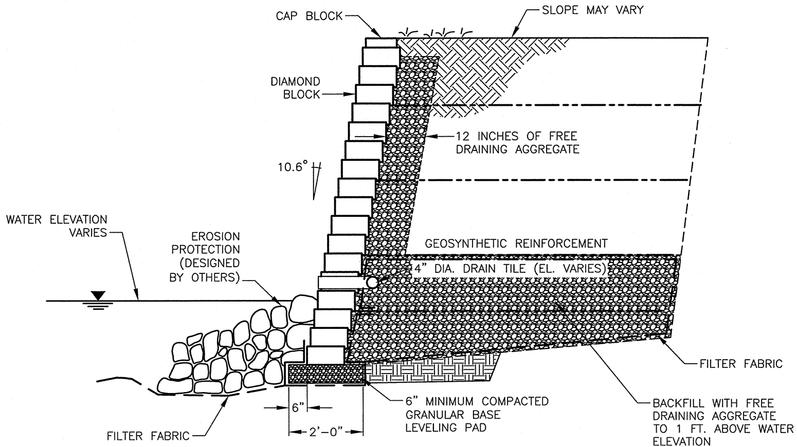
ANCHOR DIAMOND ® SHORELINE/CHANNEL WALL X WX (SCALE: 3/8" = 1'-0")
