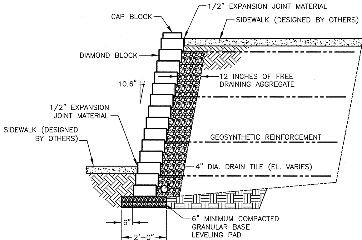
ANCHOR DIAMOND ® X SIDEWALK ABOVE/BELOW WALL WX (SCALE: 3/8" = 1'-0")
