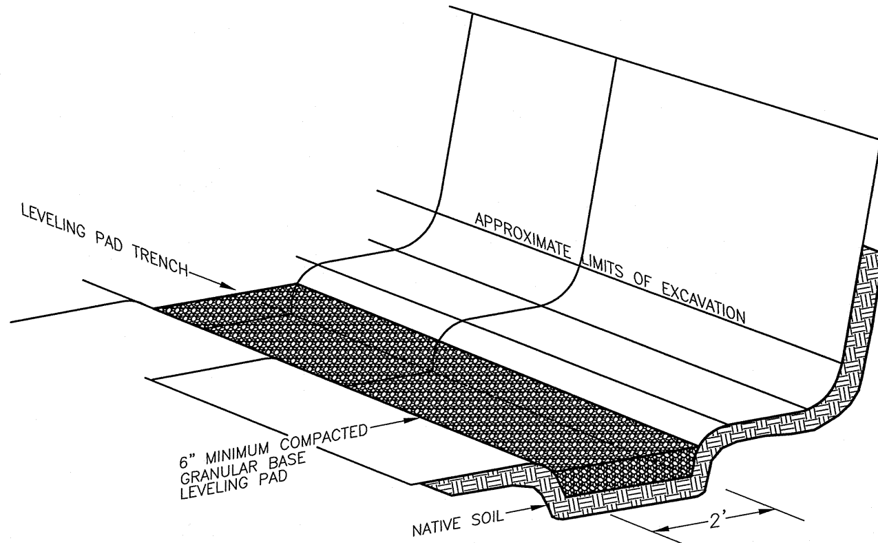
X WX ANCHOR DIAMOND ® TYPICAL BASE PREPARATION (NOT TO SCALE)
