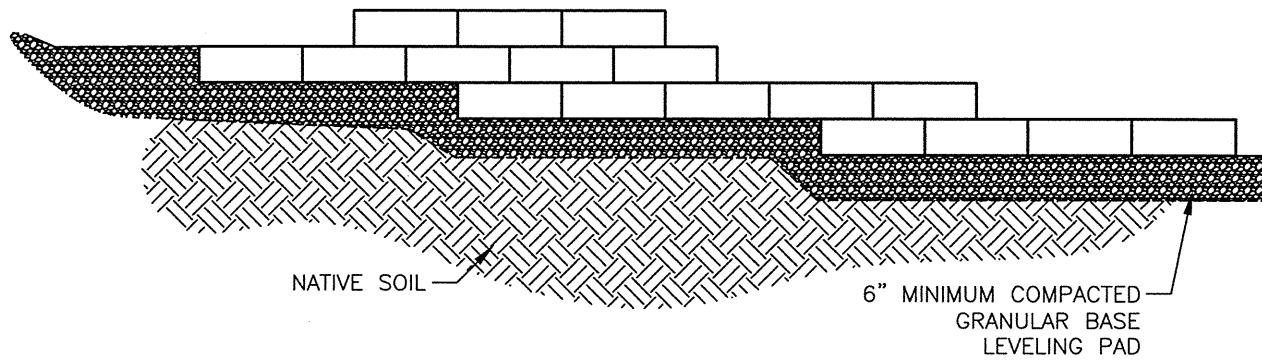
X WX ANCHOR DIAMOND ® TYPICAL STEP-UP DETAIL (NOT TO SCALE)
