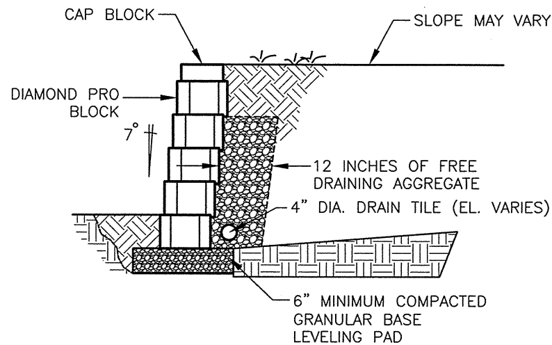
ANCHOR STONE CUT™ SERIES DIAMOND PRO™ X WX (SCALE: 3/8" = 1'-0") TYPICAL GRAVITY WALL
