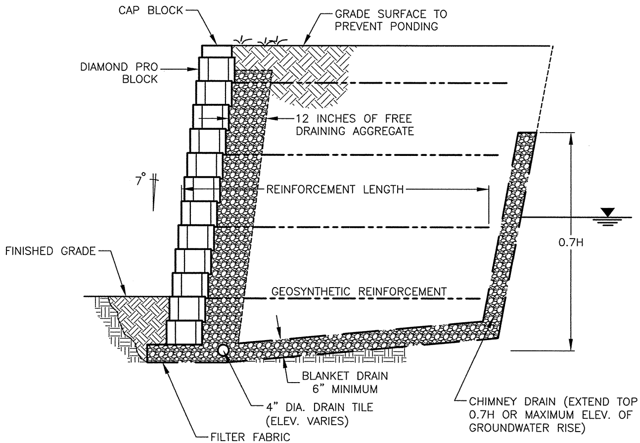
X WX (SCALE: 3/8" = 1'-0") ANCHOR STONE CUT™ SERIES DIAMOND PRO™ POTENTIAL GROUNDWATER BEHIND WALL
