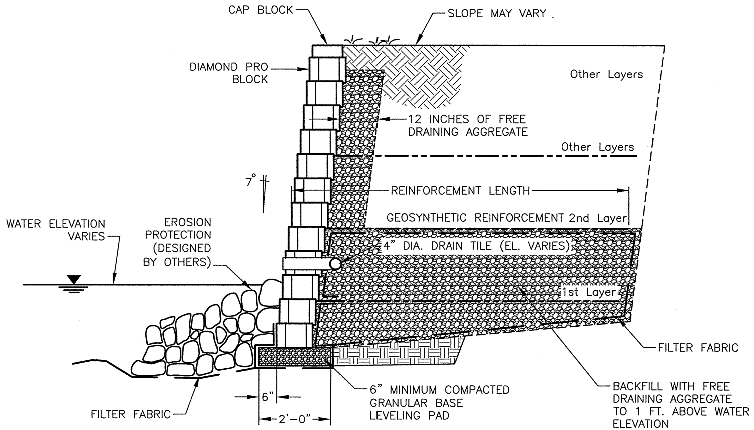
X ANCHOR STONE CUT™ SERIES DIAMOND PRO™ SHORELINE/CHANNEL WALL WX (SCALE: 3/8" = 1'-0")
