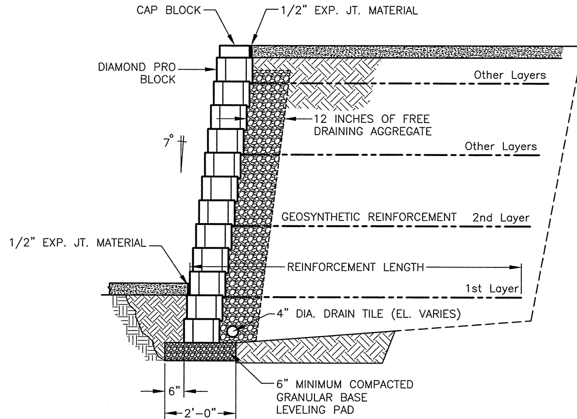
X WX (SCALE: 3/8" = 1'-0") ANCHOR STONE CUT™ SERIES DIAMOND PRO™ SIDEWALK ABOVE/BELOW WALL
