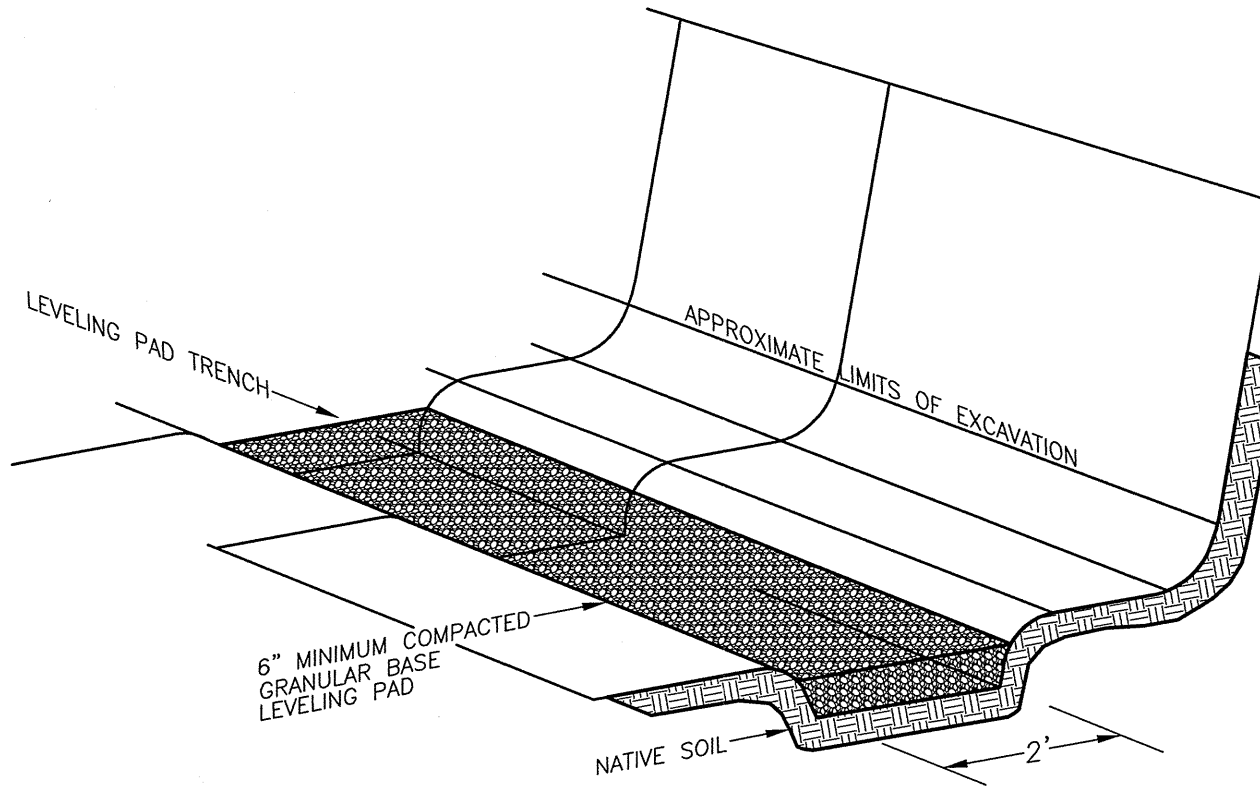
X ANCHOR STONE CUT™ SERIES DIAMOND PRO™ TYPICAL BASE PREPARATION WX (NOT TO SCALE)
