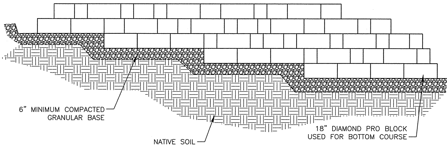
X WX ANCHOR STONE CUT™ SERIES DIAMOND PRO™ TYPICAL STEP-UP DETAIL (NOT TO SCALE)
