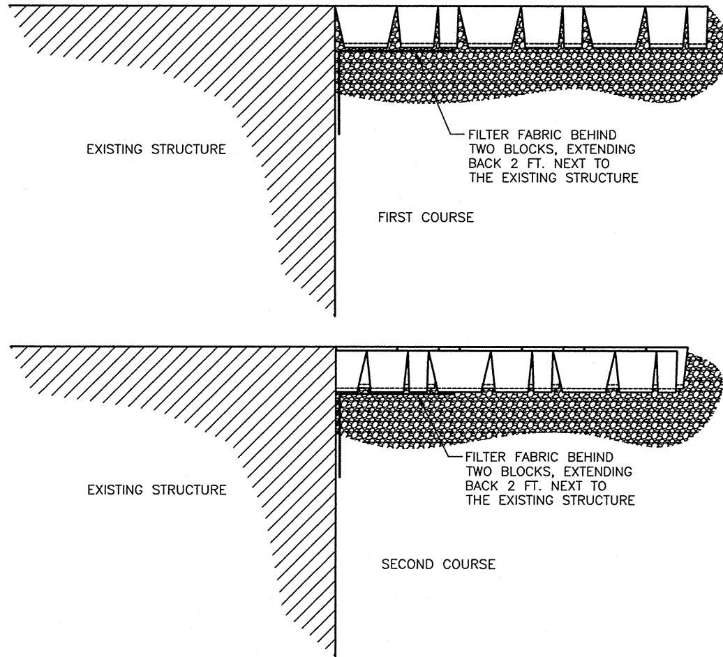
ANCHOR HIGHLAND STONE™ X WALL ABUTTING EXISTING STRUCTURE WX (NOT TO SCALE)
