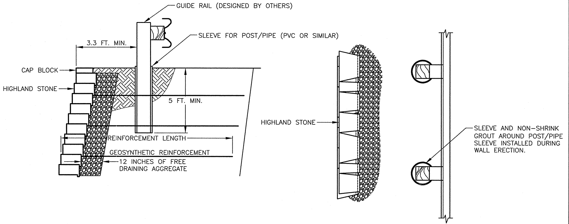
ANCHOR HIGHLAND STONE™ X GUIDE RAIL DETAIL WX (NOT TO SCALE)
