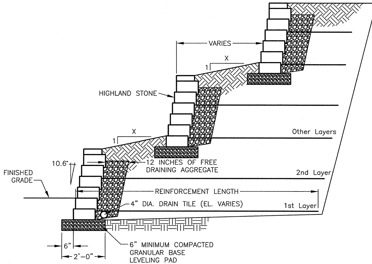
X ANCHOR HIGHLAND STONE™ TERRACED WALL WX (NOT TO SCALE)
