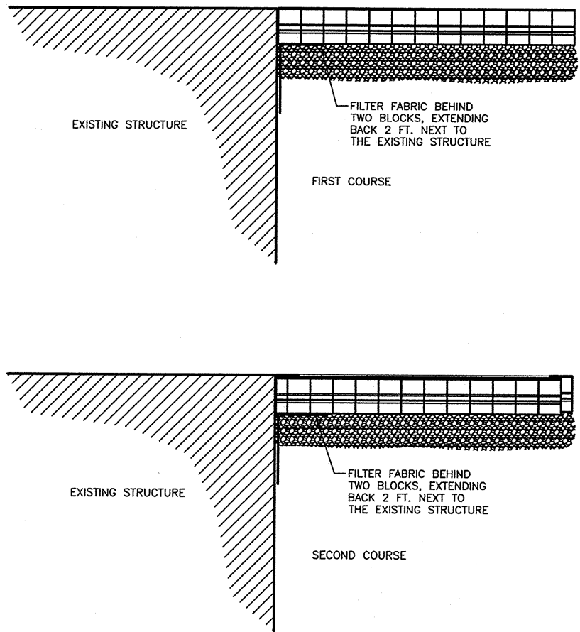
X ANCHOR LANDMARK SYSTEM WX WALL ABUTTING EXISTING STRUCTURE (NOT TO SCALE)
