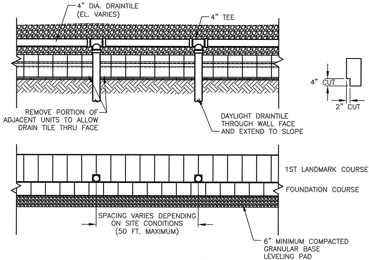
X WX (NOT TO SCALE) ANCHOR LANDMARK SYSTEM DAYLIGHT DRAINTILE THROUGH TOE SLOPE
