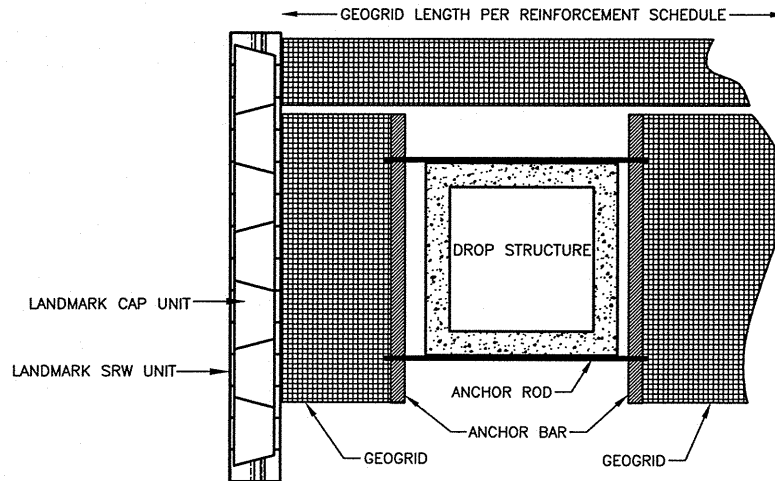
ANCHOR LANDMARK SYSTEM X DROP STRUCTURE IN REINFORCED ZONE WX (NOT TO SCALE)
