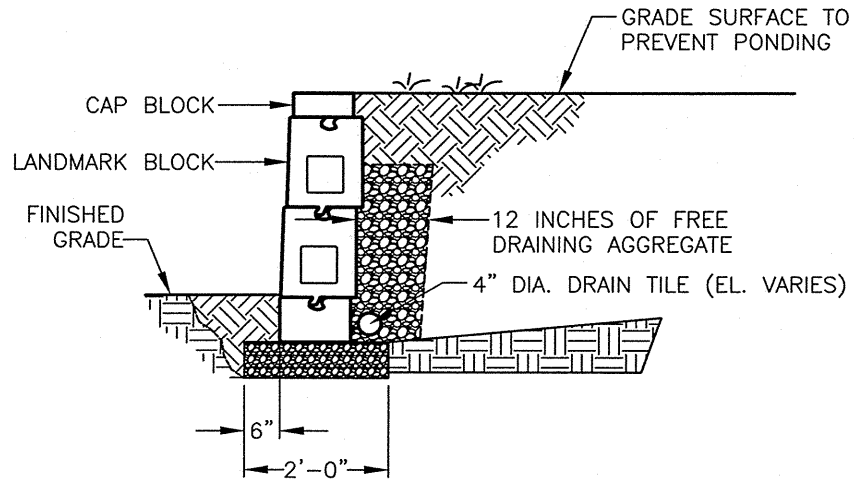
X WX ANCHOR LANDMARK SYSTEM GRAVITY WALL (SCALE: 3/8" = 1'-0")
