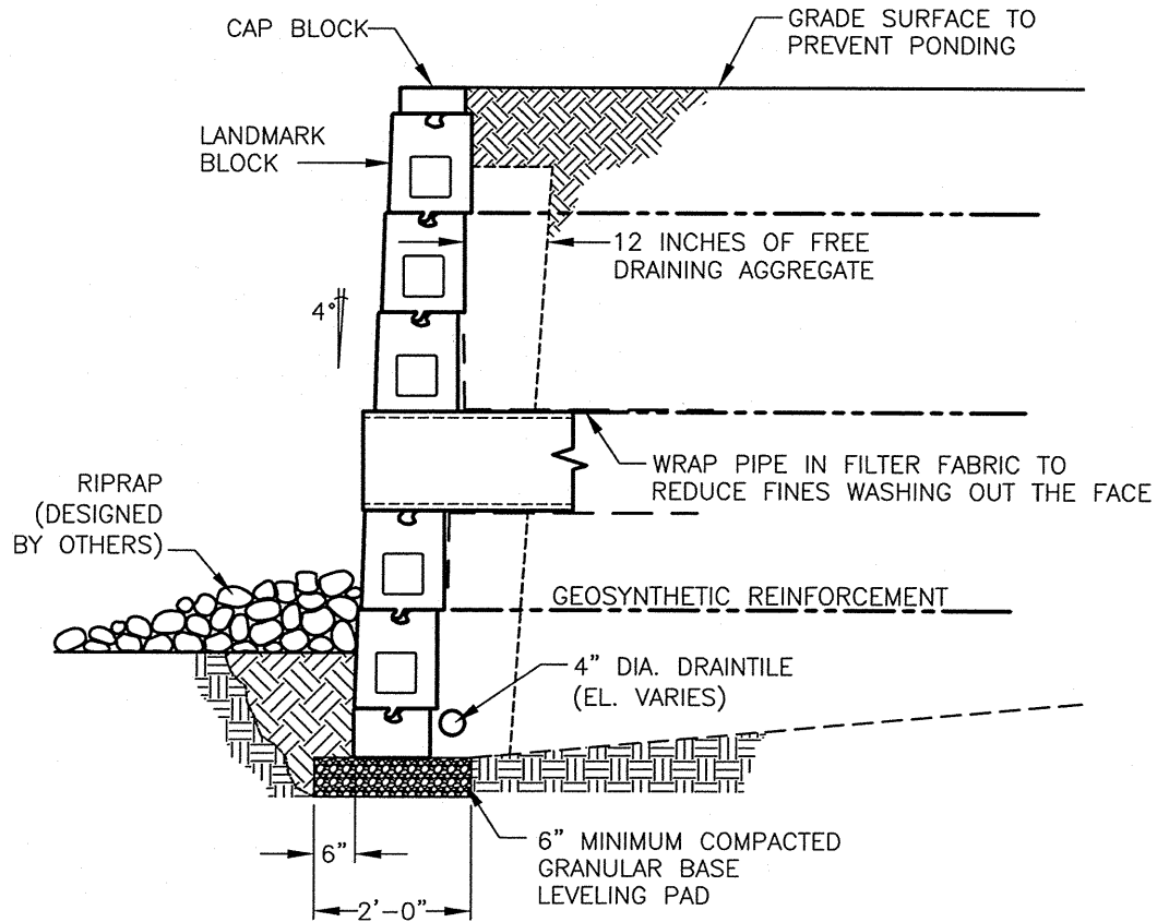
SECTION VIEW
