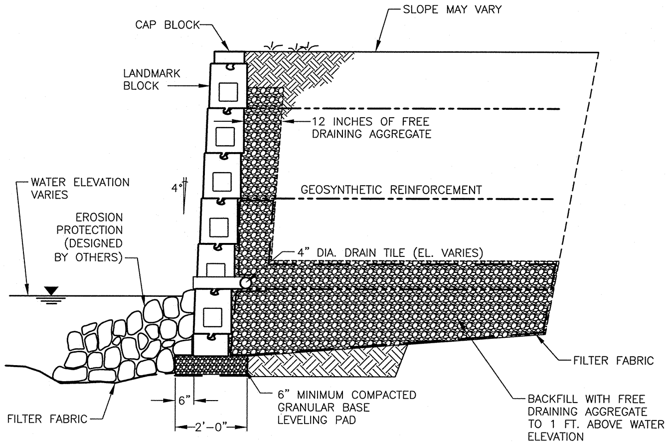
X WX ANCHOR LANDMARK SYSTEM SHORELINE/CHANNEL WALL (SCALE: 3/8" = 1'-0")
