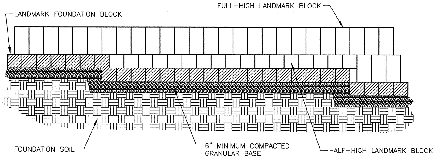
X ANCHOR LANDMARK SYSTEM TYPICAL STEP-UP DETAIL WX (NOT TO SCALE)
