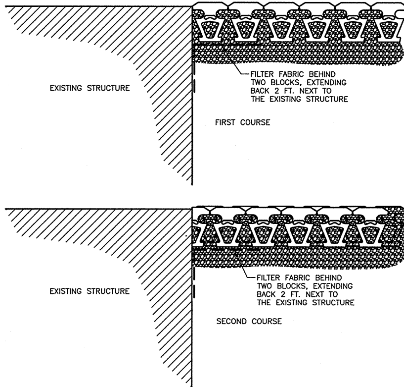
ANCHOR VERTICA PRO® WALL ABUTTING EXISTING STRUCTURE (NOT TO SCALE)
