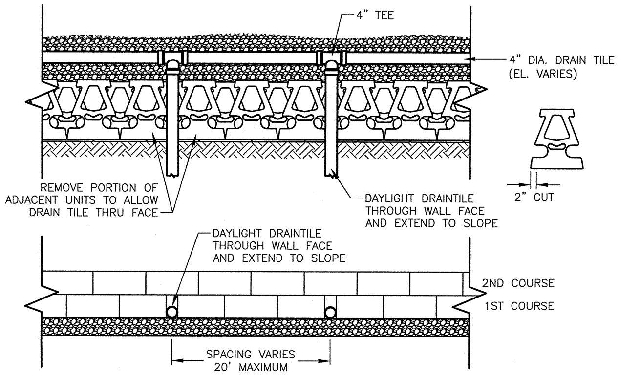
X ANCHOR VERTICA PRO® WX DAYLIGHT DRAINTILE THROUGH TOE SLOPE (NOT TO SCALE)
