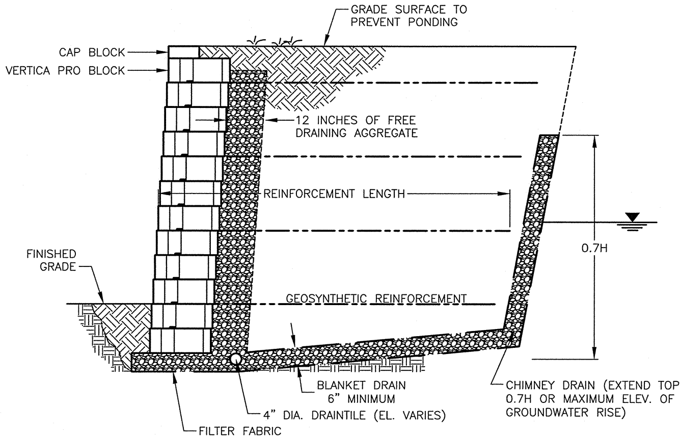
ANCHOR VERTICA PRO ® POTENTIAL GROUNDWATER BEHIND WALL (SCALE: 3/8" = 1'-0")
