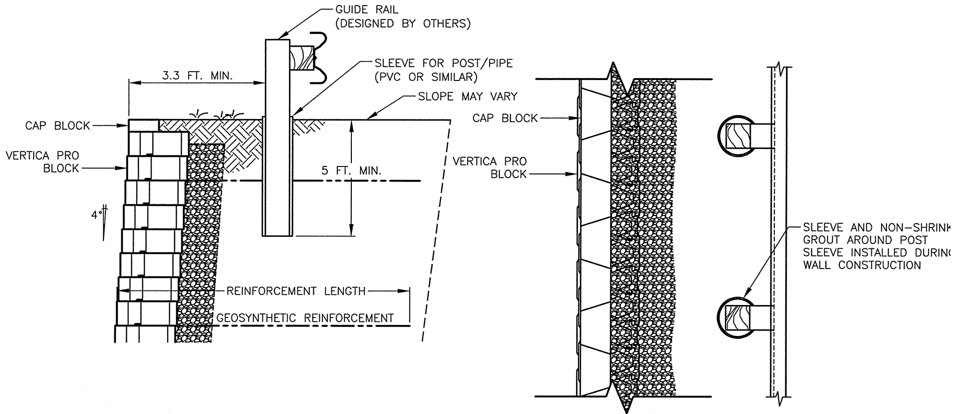
X WX ANCHOR VERTICA PRO® GUIDE RAIL DETAIL (NOT TO SCALE)
