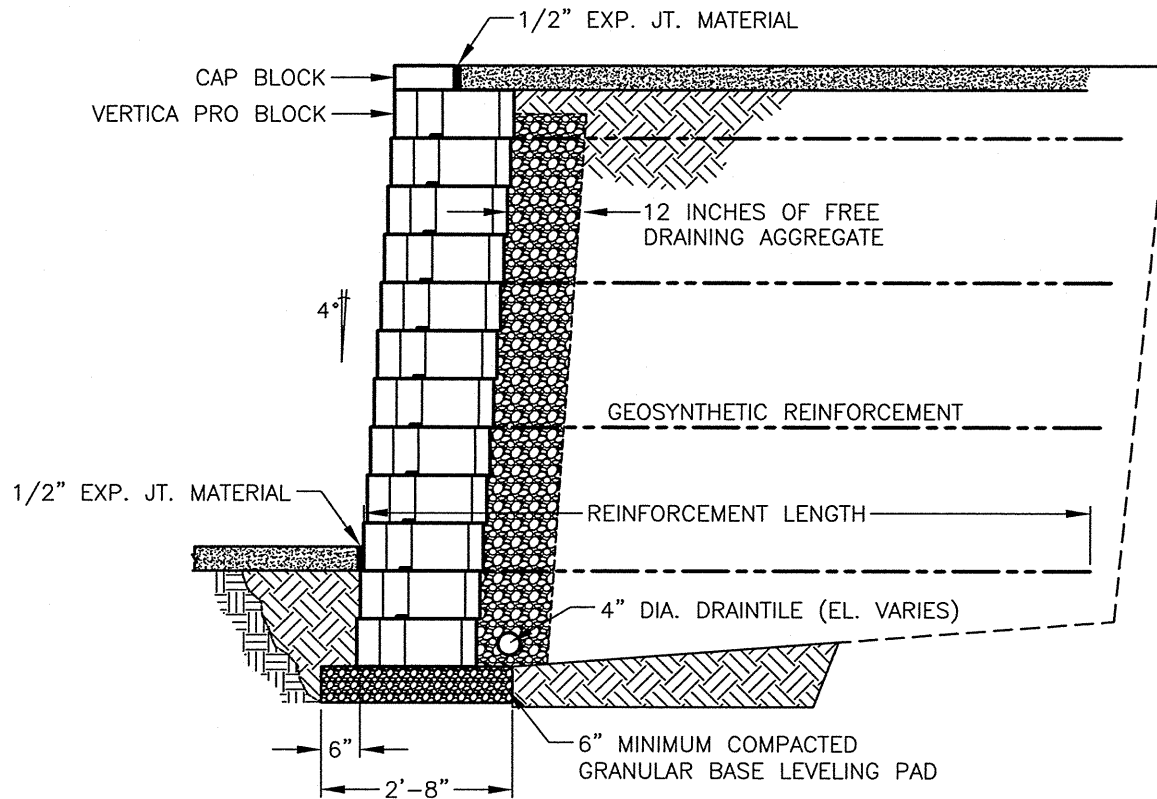
X ANCHOR VERTICA PRO® WX SIDEWALK ABOVE/BELOW WALL (SCALE: 3/8" = 1'-0")
