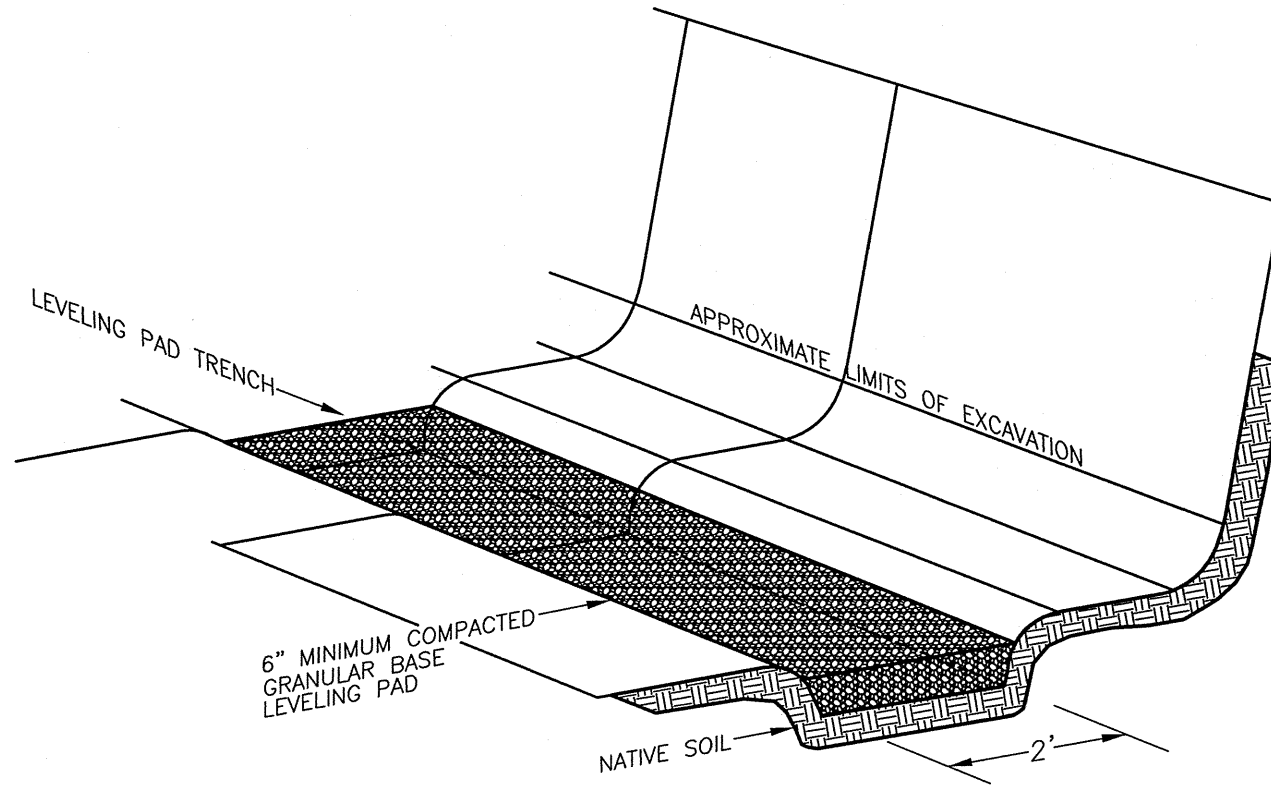
X WX ANCHOR VERTICA PRO ® TYPICAL BASE PREPARATION (NOT TO SCALE)
