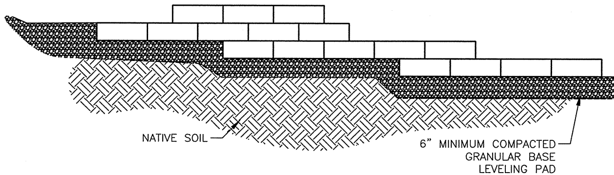
X ANCHOR VERTICA PRO® WX TYPICAL STEP-UP DETAIL (NOT TO SCALE)
