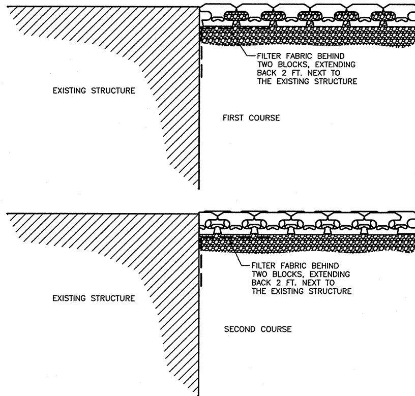
X WX ANCHOR VERTICA® WALL ABUTTING EXISTING STRUCTURE (NOT TO SCALE)
