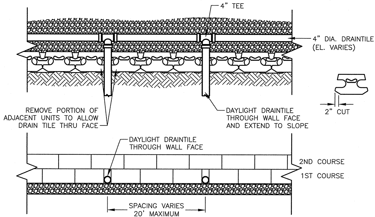
ANCHOR VERTICA ® X DAYLIGHT DRAINTILE THROUGH TOE SLOPE WX (NOT TO SCALE)
