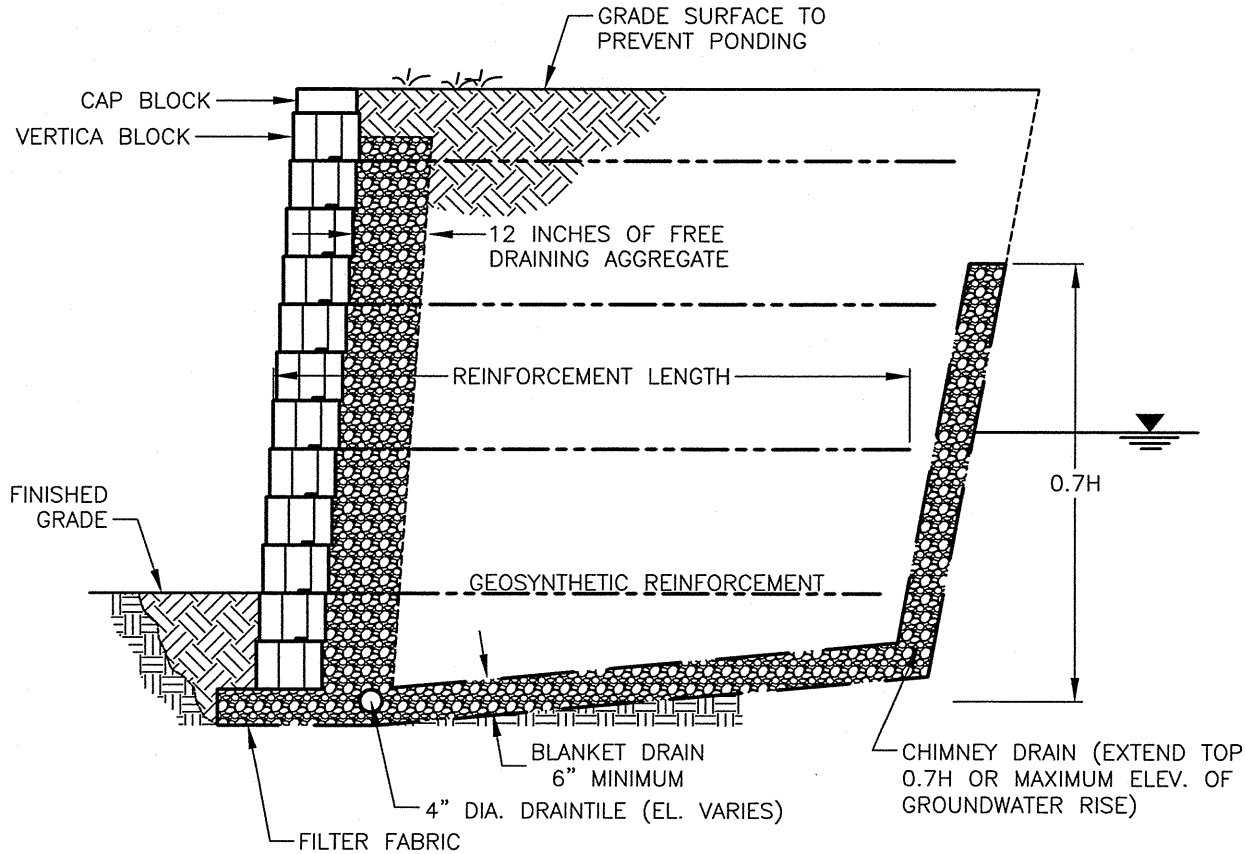
ANCHOR VERTICA® POTENTIAL GROUNDWATER BEHIND WALL (SCALE: 3/8" = 1'-0")
