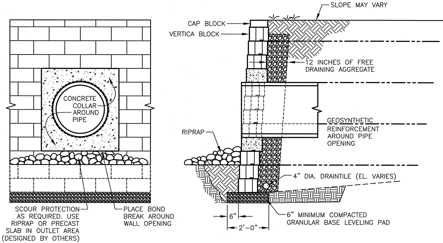
SECTION VIEW
