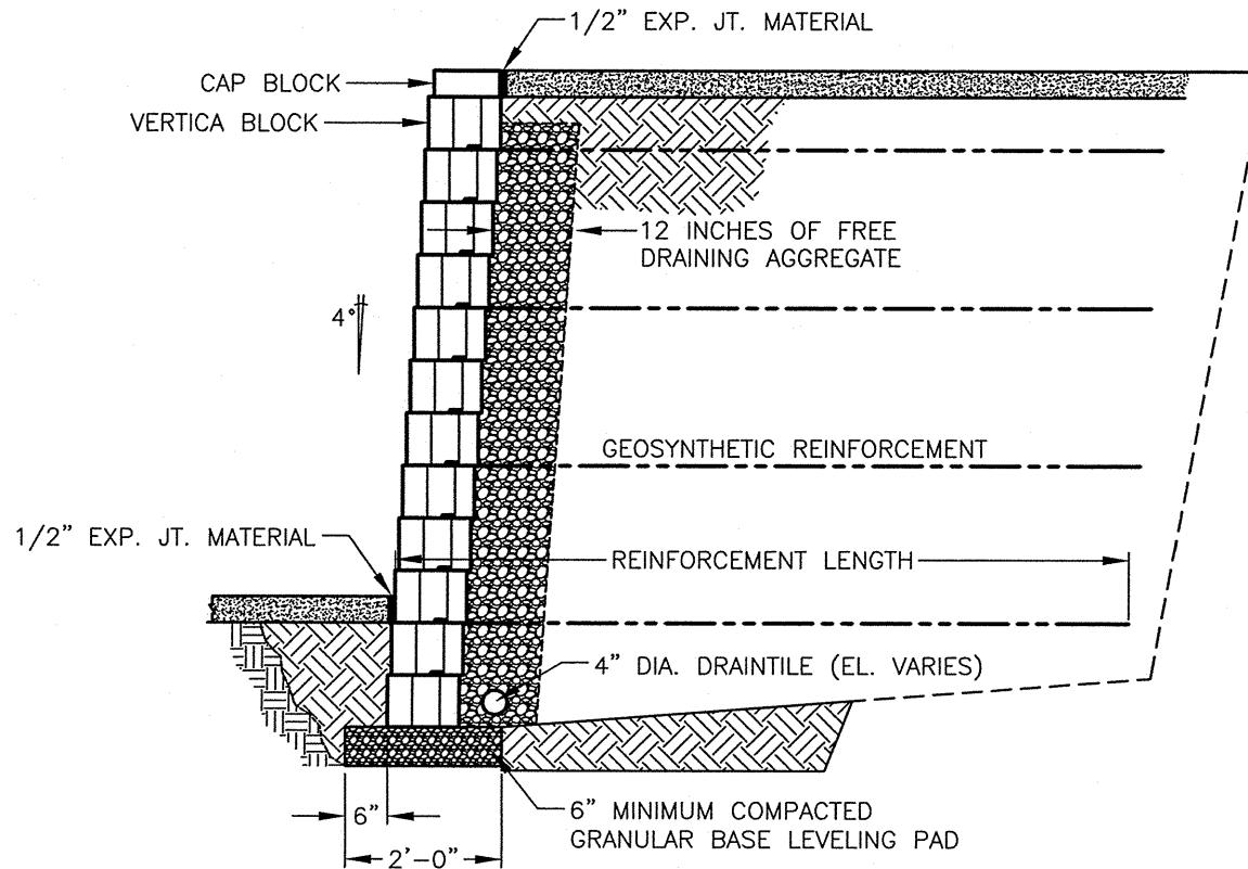
ANCHOR VERTICA® X SIDEWALK ABOVE/BELOW WALL WX (SCALE: 3/8" = 1'-0")
