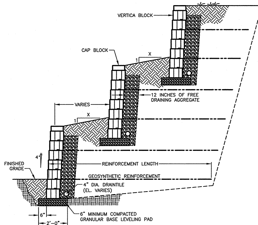
X WX ANCHOR VERTICA® TERRACED WALLS DETAIL (NOT TO SCALE)
