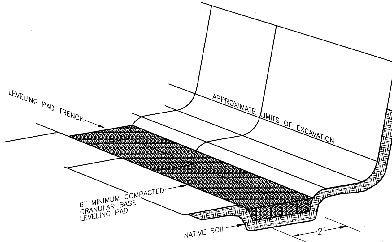
X ANCHOR VERTICA ® TYPICAL BASE PREPARATION WX (NOT TO SCALE)
