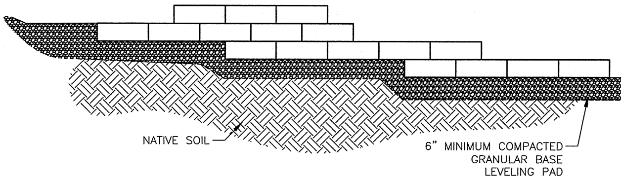
ANCHOR VERTICA ® X TYPICAL STEP-UP DETAIL WX (NOT TO SCALE)
